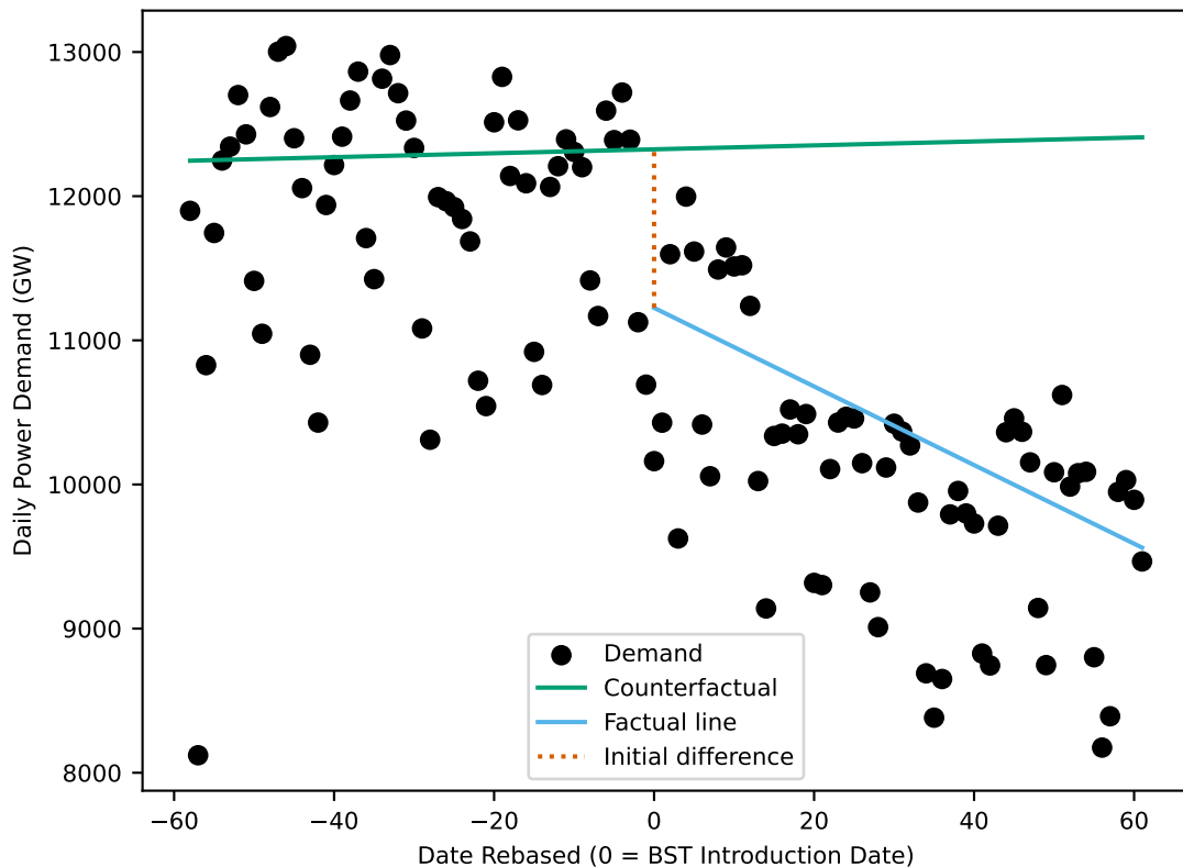
Power Demand Regressions Around Clock Change 2013
