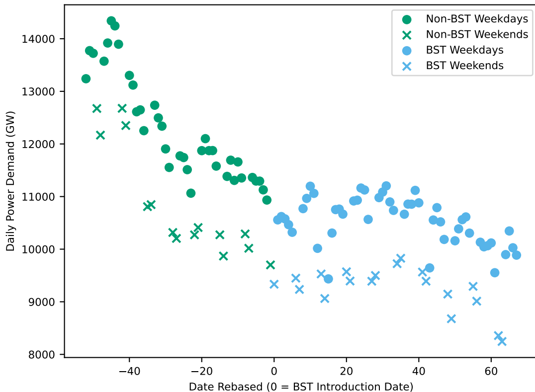
Power Demand Around Clock Change 2012
