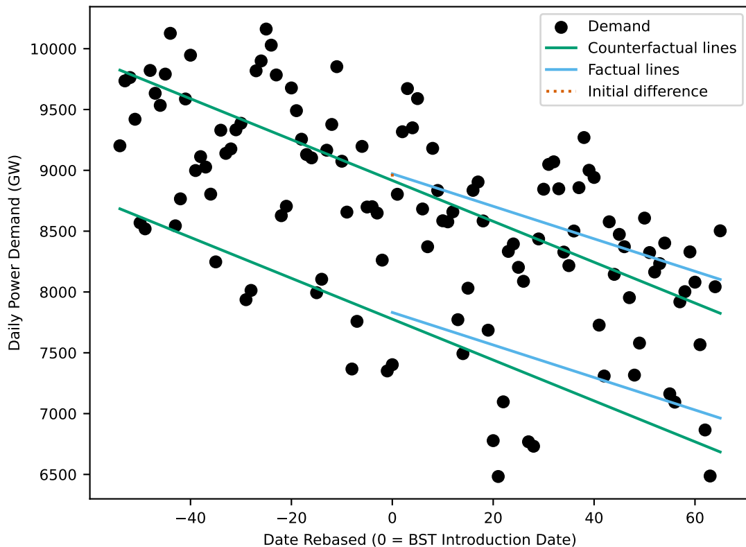
Power Demand Regressions Around Clock Change 2022
