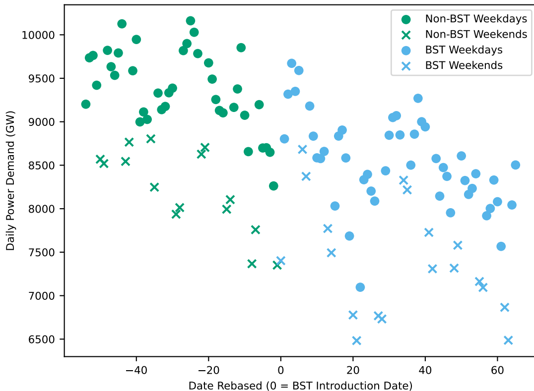
Power Demand Around Clock Change 2022
