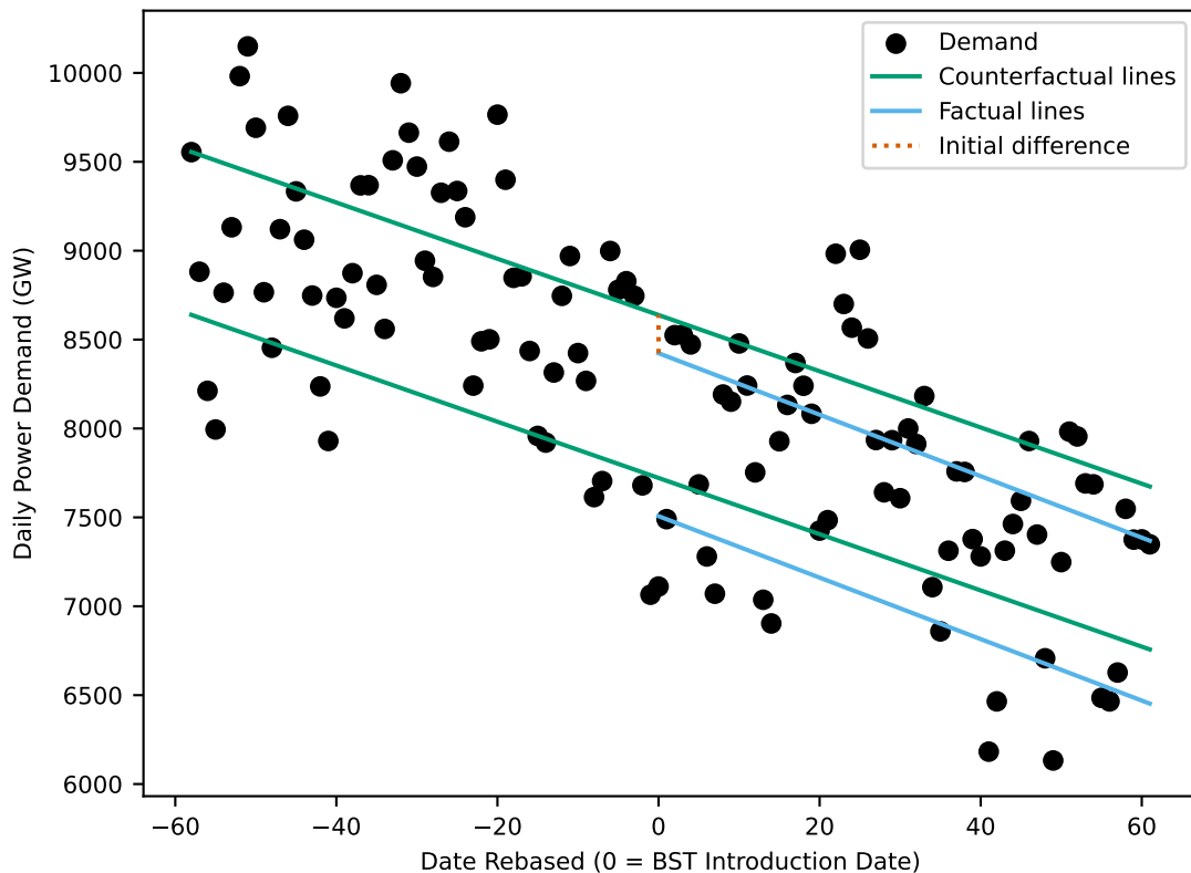
Power Demand Regressions Around Clock Change 2024
