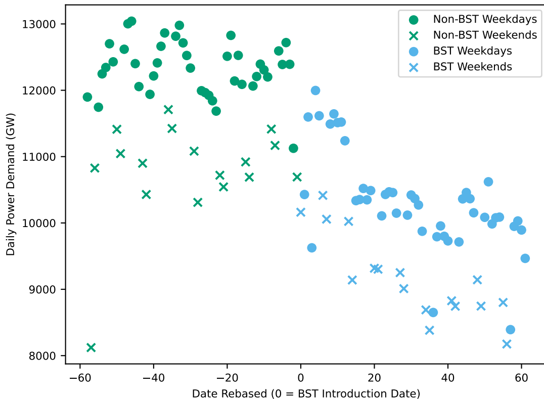
Power Demand Around Clock Change 2013
