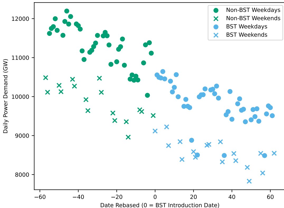
Power Demand Around Clock Change 2014
