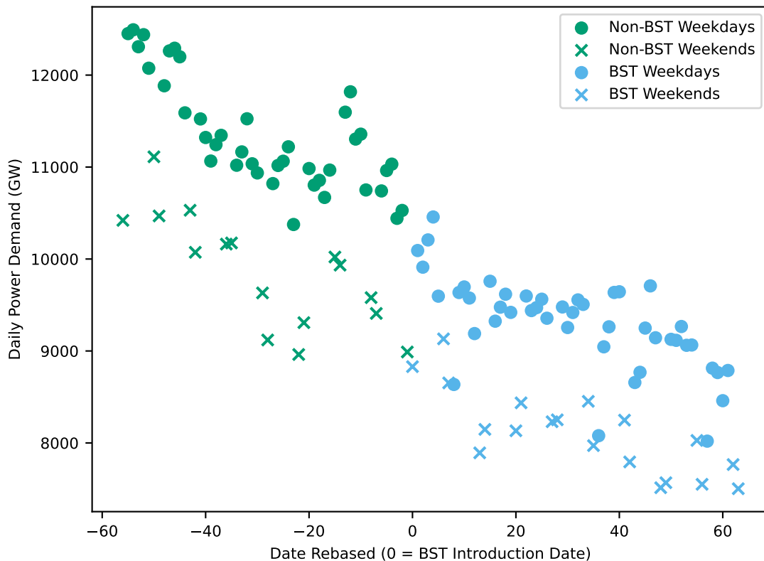
Power Demand Around Clock Change 2015
