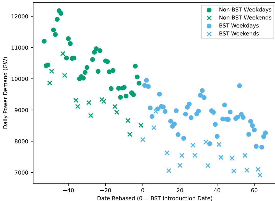
Power Demand Around Clock Change 2017
