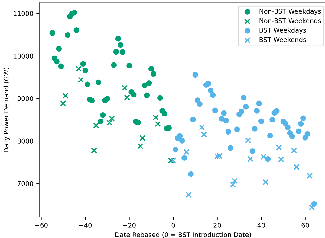
Power Demand Around Clock Change 2021
