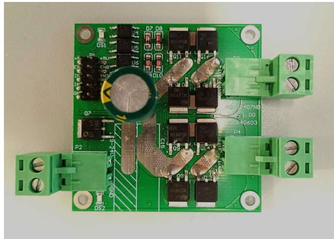
Figura 2.12: Driver AQMH2407ND
