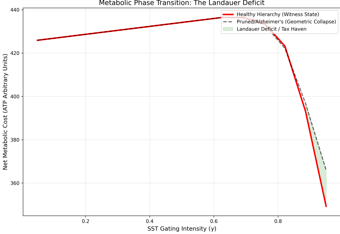
Figure 5: The Metabolic Energy ROI. Simulation of total metabolic cost ( C_{Total} ) as a function of SST gating intensity ( \gamma ). Red Line: Healthy hierarchical networks undergo a phase transition at \gamma \approx 0.8 , accessing a “Signaling Tax Haven” where geodesic shortcuts reduce net energy consumption despite high integration. Grey Line: Pathological networks (30% synaptic pruning) suffer “Geometric Collapse,” failing to access the transition and incurring a linear metabolic penalty (the Landauer Wall). Green Region: The “Landauer Deficit”—the explicit energetic advantage of the Witness State [17].
