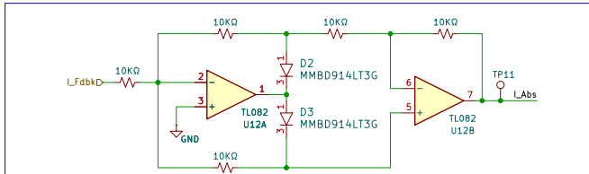
ABSOLUTE CURRENT GENERATOR
