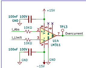
REFERENCE TO ABSOLUTE CURRENT COMPARATOR
