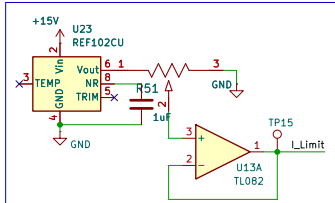
REFERENCE CURRENT VOLTAGE FOLLOWER
