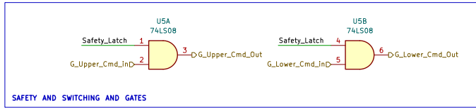
SAFETY AND SWITCHING AND GATES
