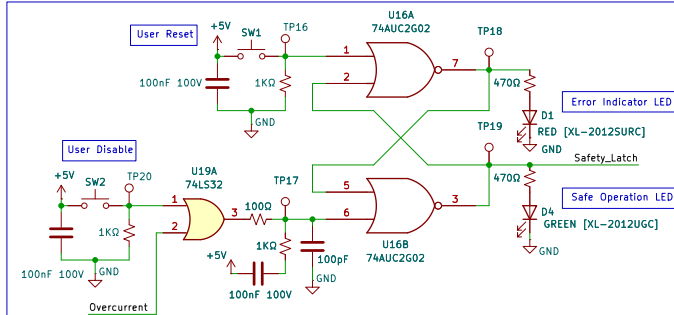
CURRENT SAFETY FLIP_FLOP AND USER MANUAL RESET
