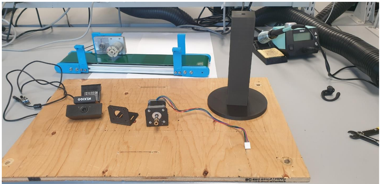
Figure 5: Mounted hardware (In progress)
