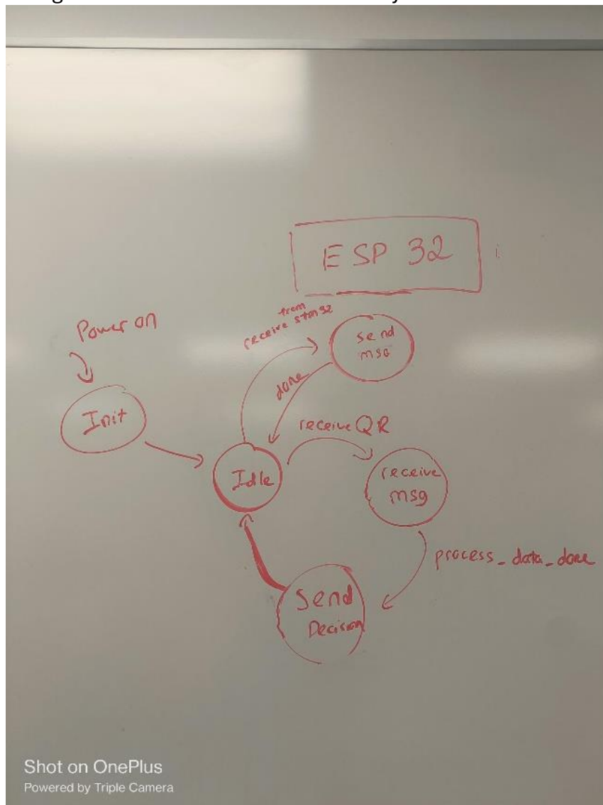
Figure 1: State machine for ESP32
