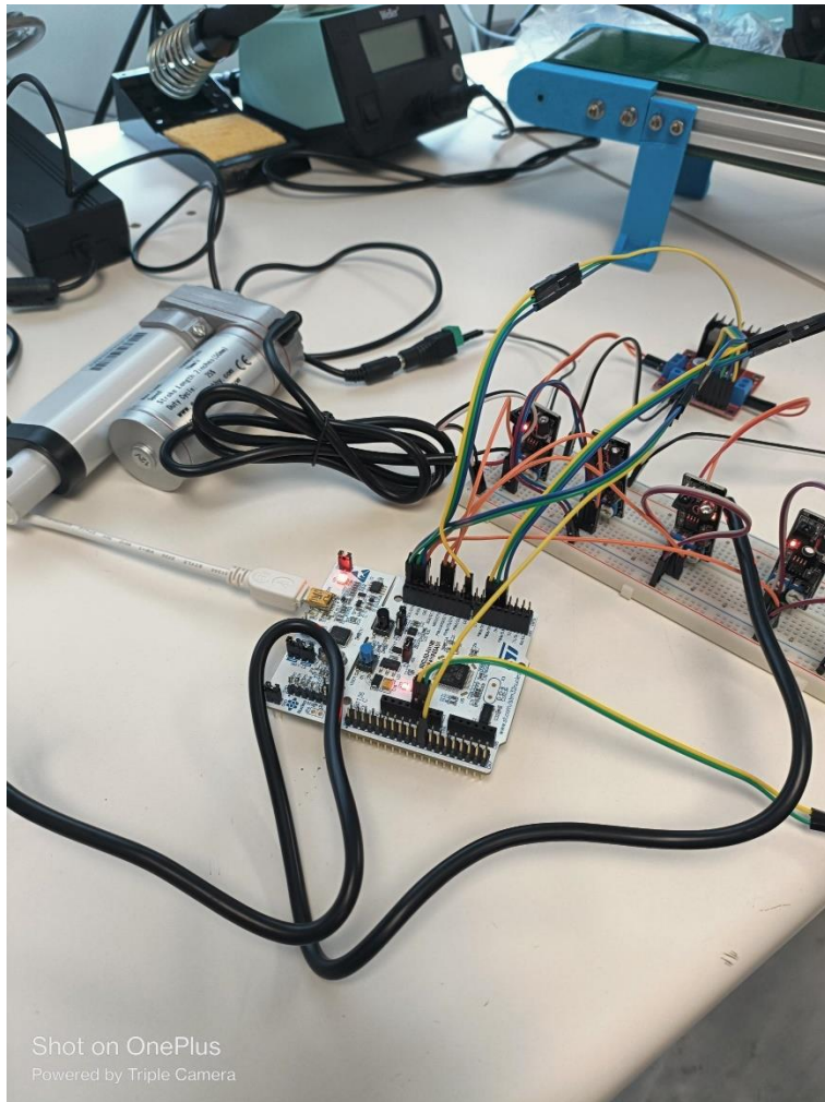
Figure 2: STM32 connections
