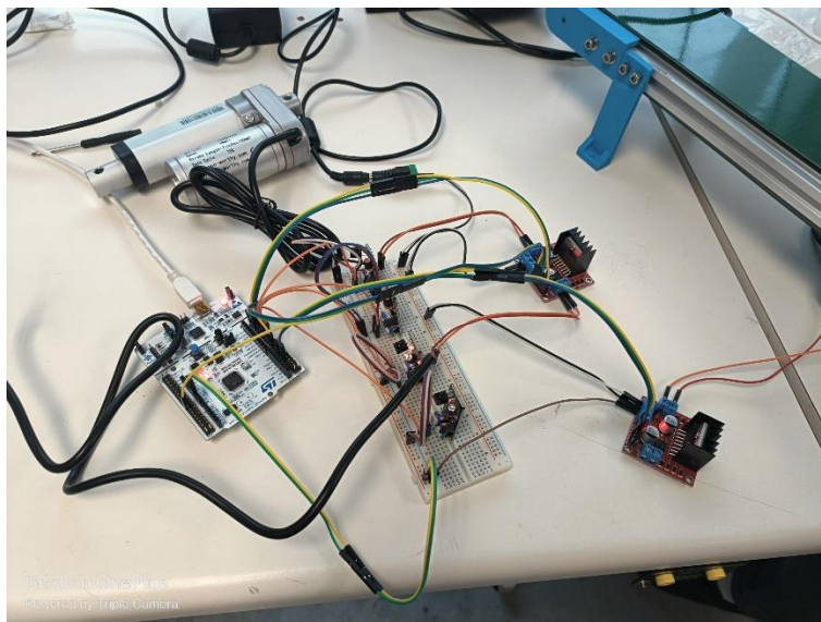
Figure 4: Full components wiring
