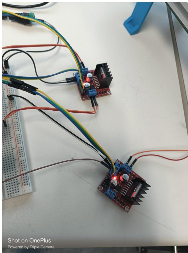
Figure 1: L298 driver connection
