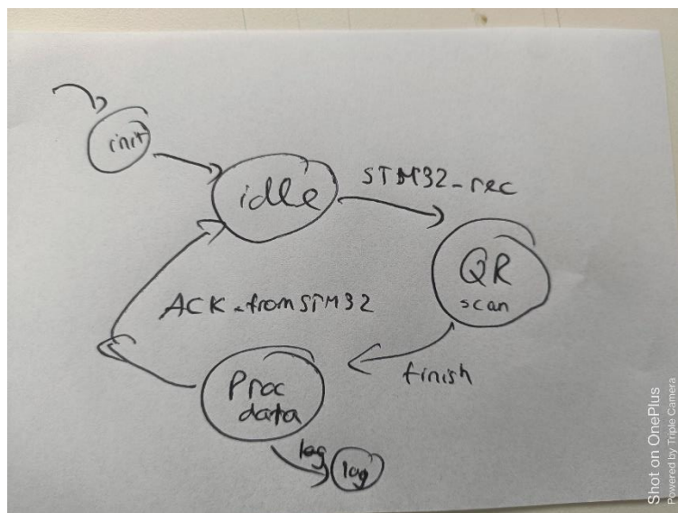
Figure 2: Raspberry Pi 4's state machine
