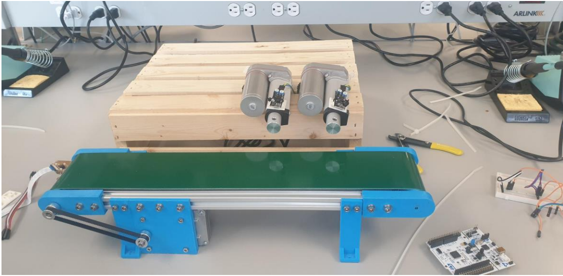
Figure 5: Mounted hardware (In progress)
