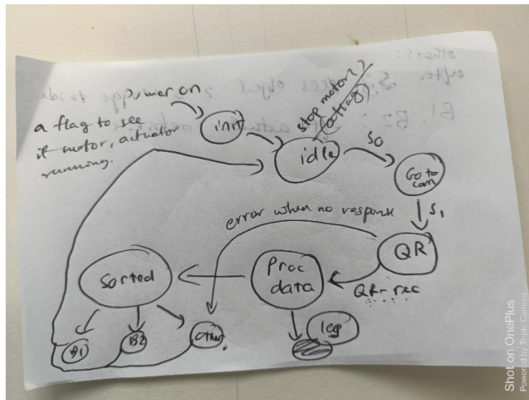
Figure 1: STM32's state machine
