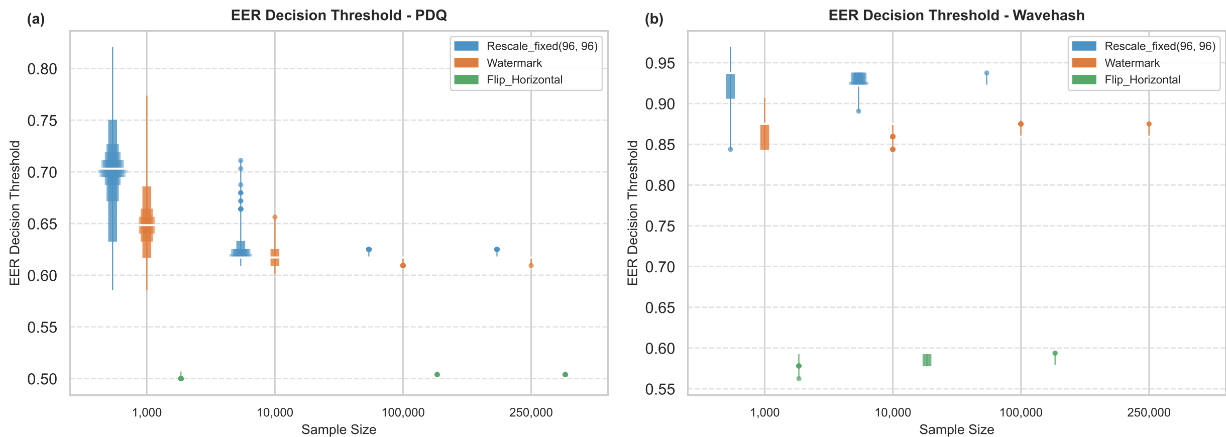
Fig. 4. Metric convergence for EER thresholds for three transforms. Note that the plots do not share the y-axis.
