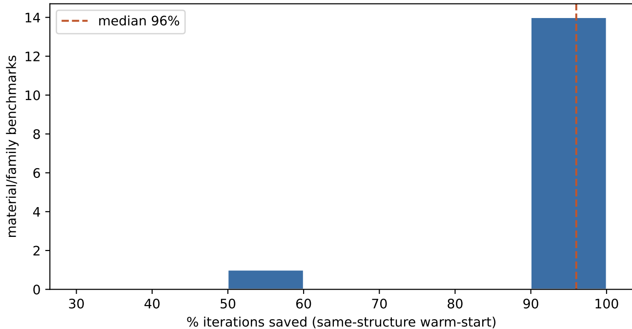
Distribution of warm-start iteration savings
