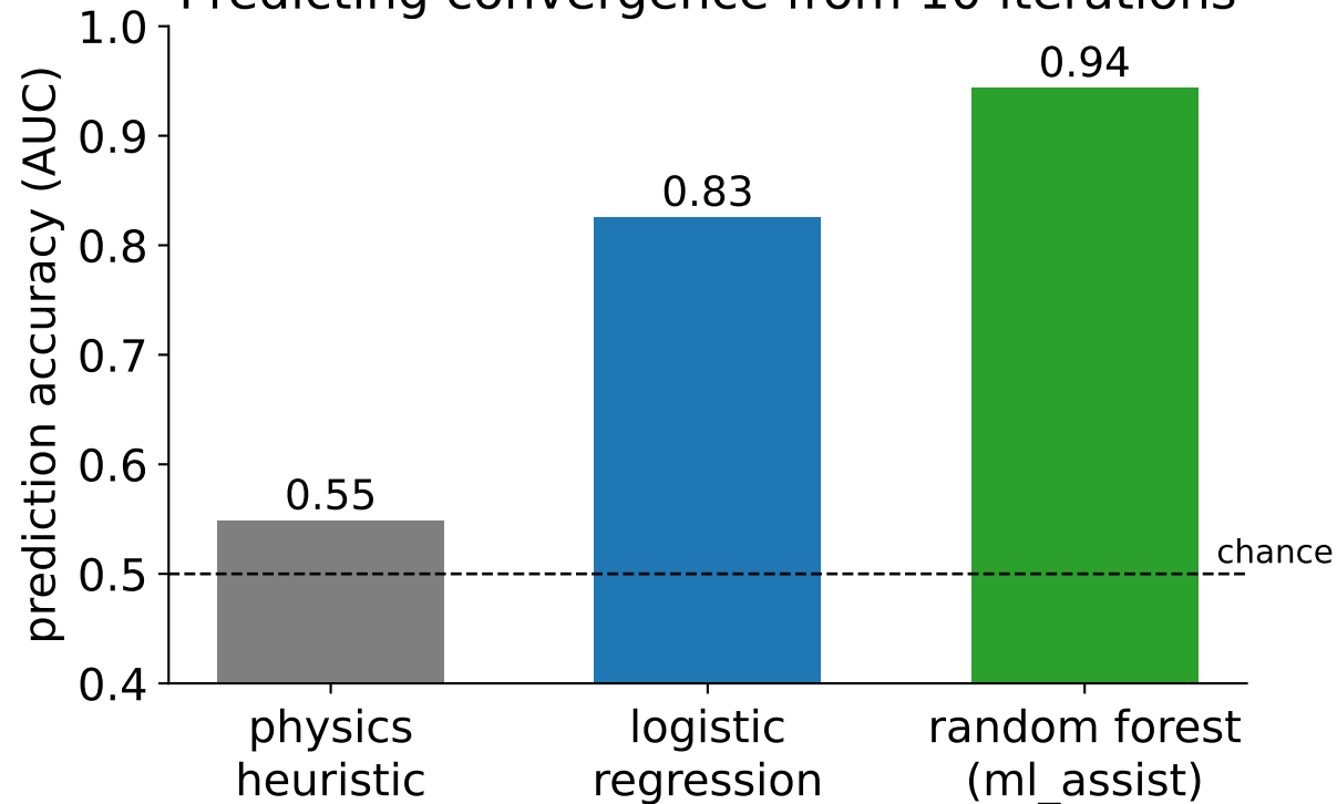
Predicting convergence from 10 iterations
