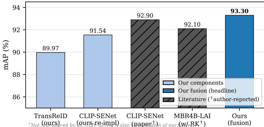
VeRi-776 mAP Comparison
