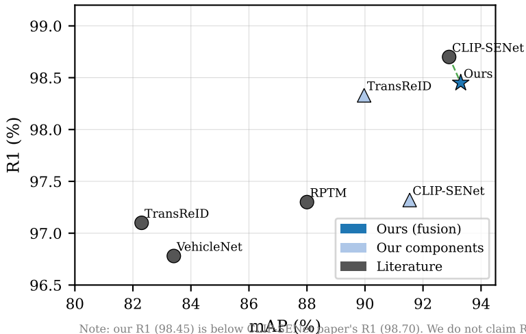
VeRi-776 R1 vs. mAP
