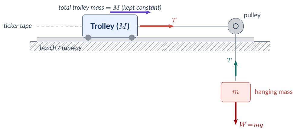
Figure E2.1 – Trolley connected by string over a pulley to a hanging mass. The hanging mass provides the driving force; the pulley redirects the tension.
