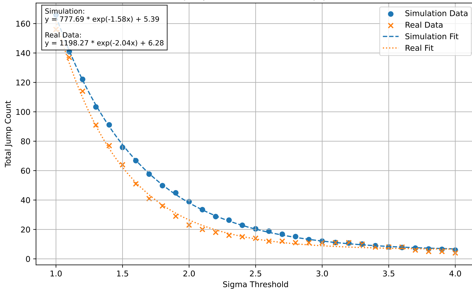
Jump Calibration Curve Fit: JNJ
