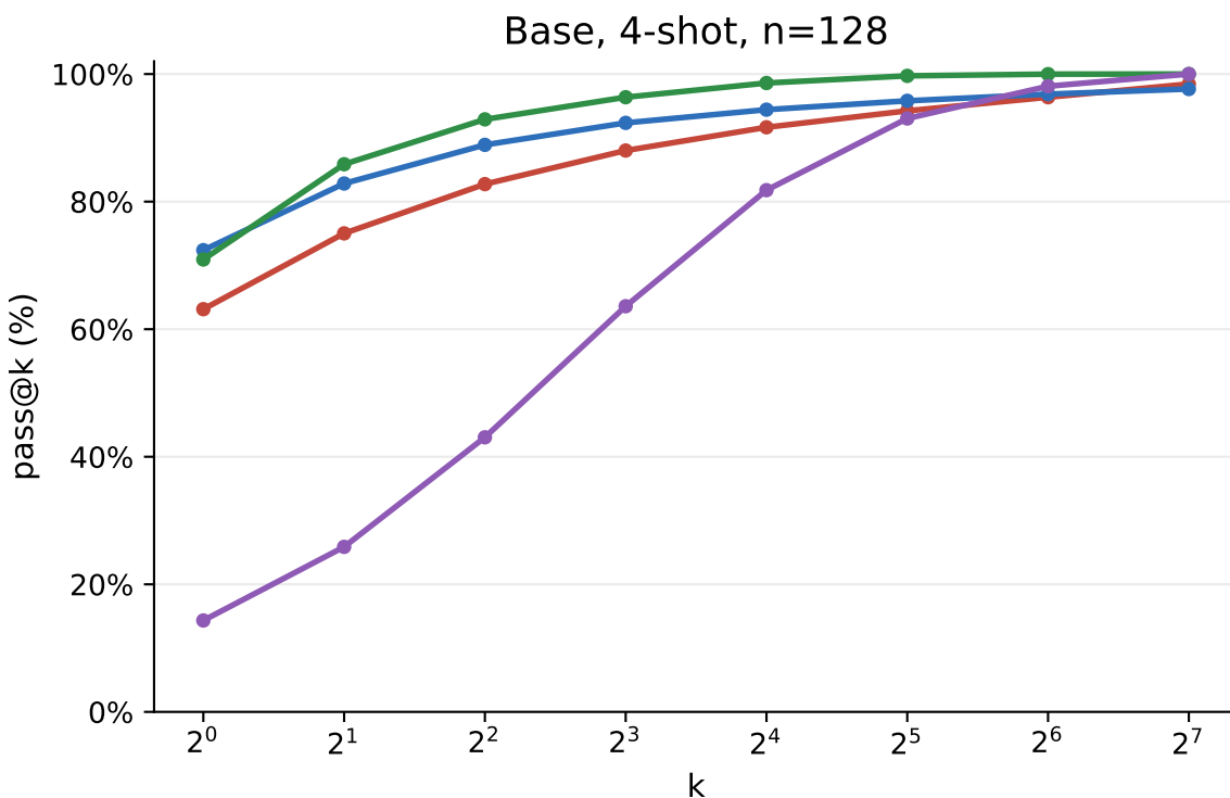
GSM8K pass@k across prompt and few-shot settings
