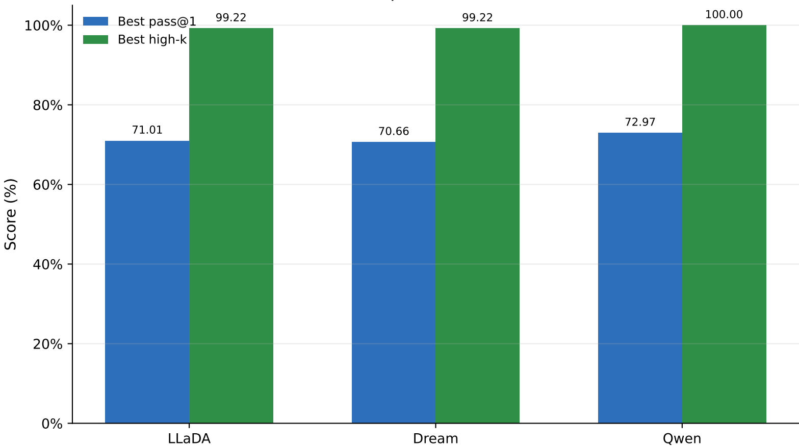
GSM8K sweep best observed scores
