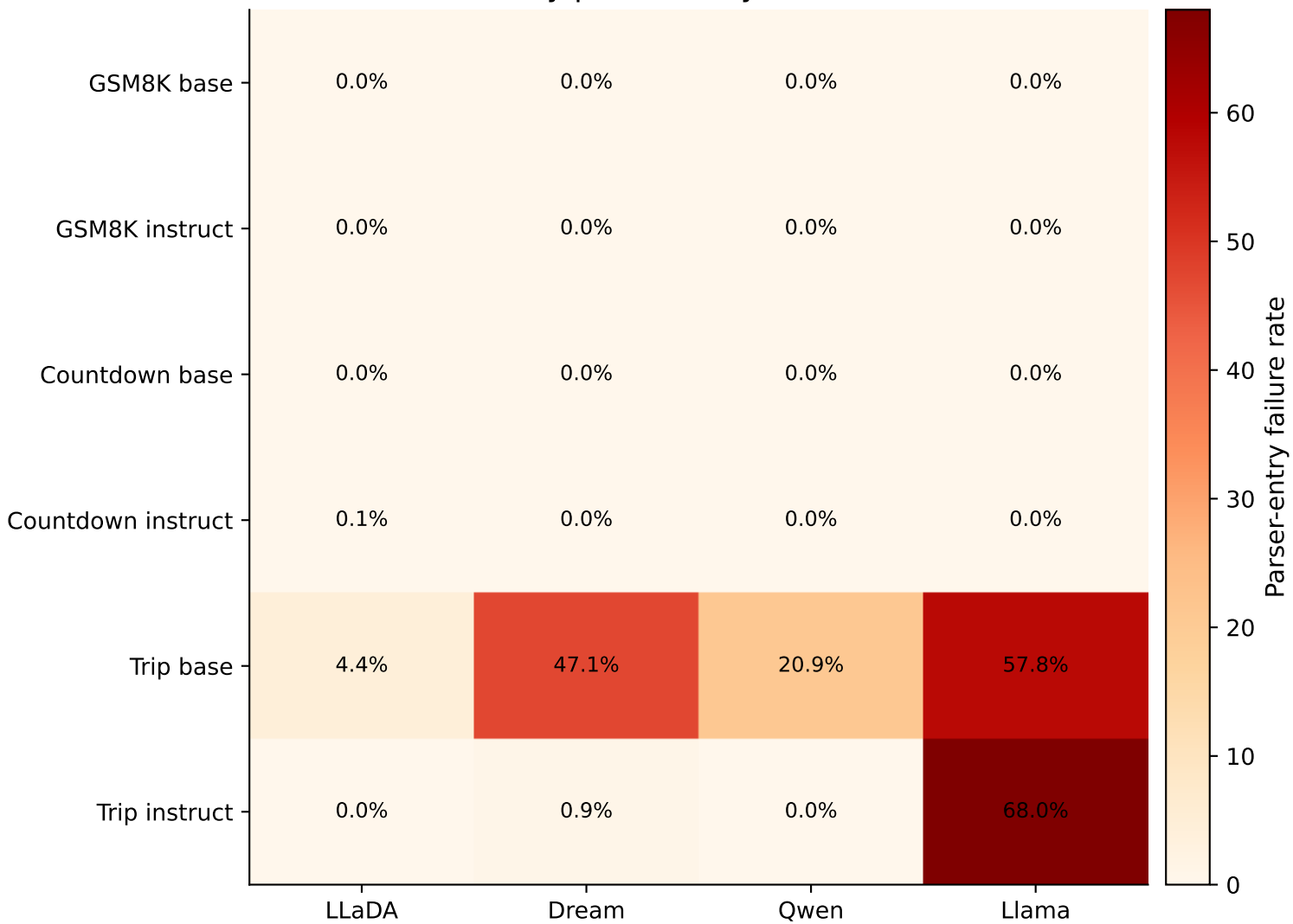
Primary parser-entry failure rates
