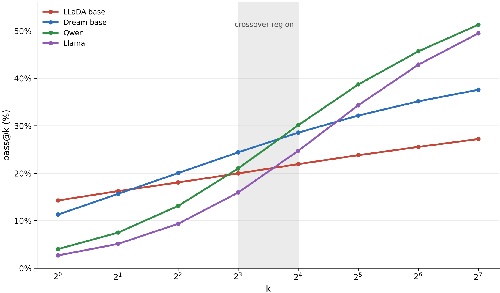
Countdown-cd4 base pass@k crossover
