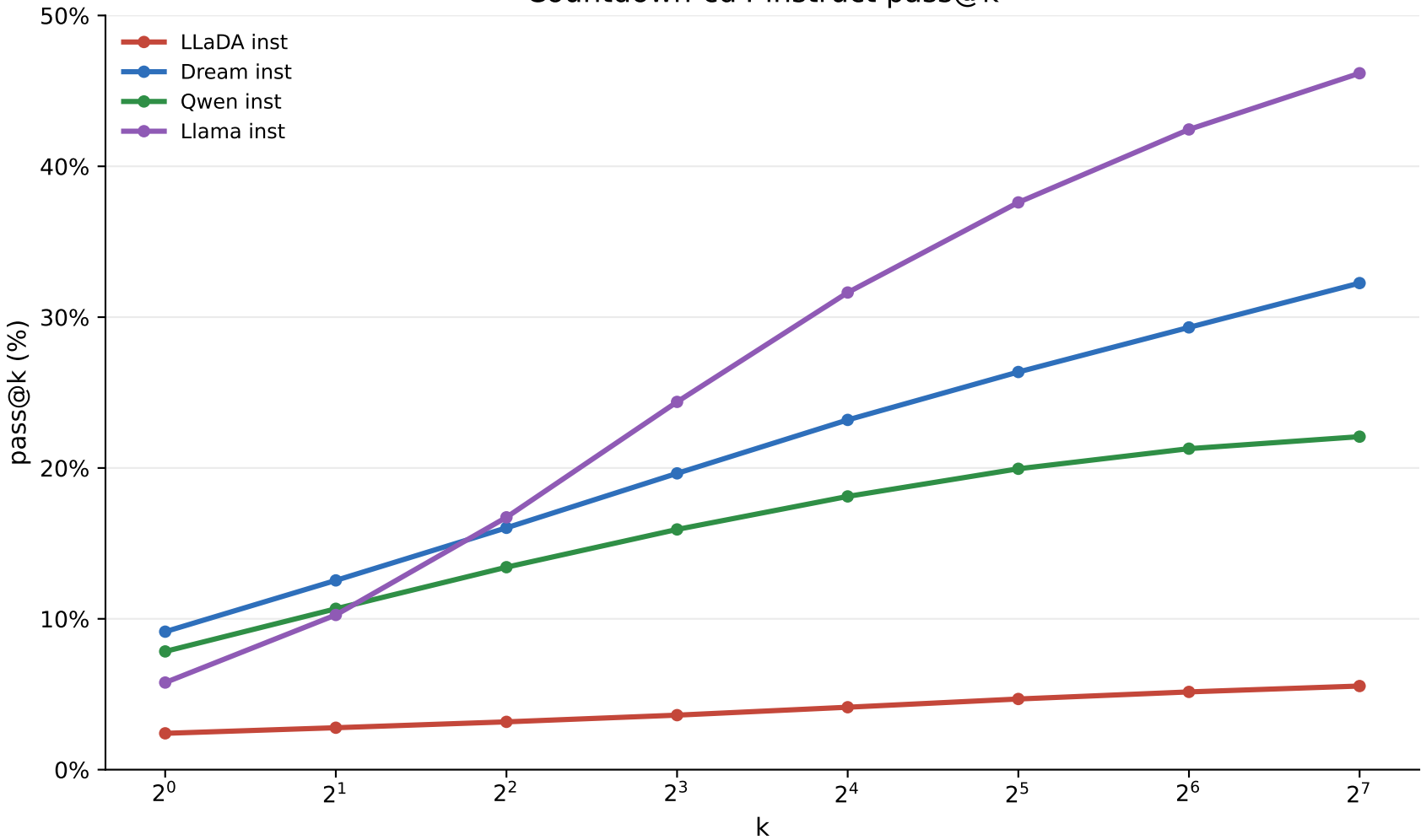
Countdown-cd4 instruct pass@k
