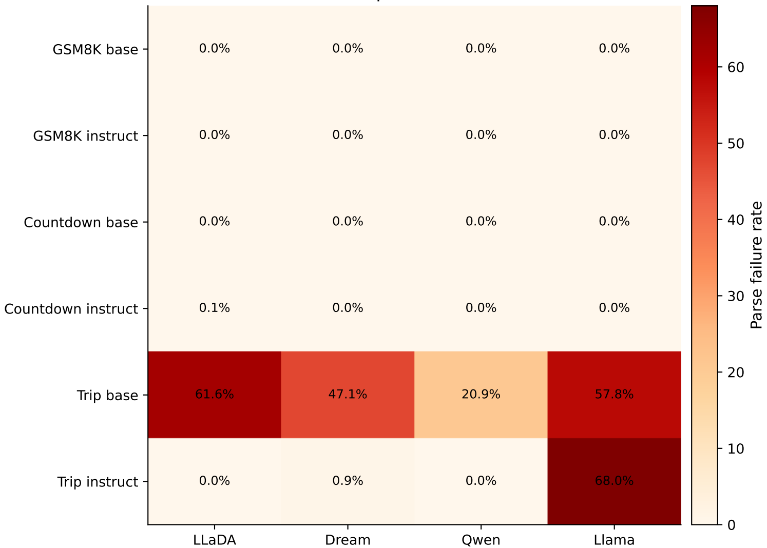
Canonical parser failure rates
