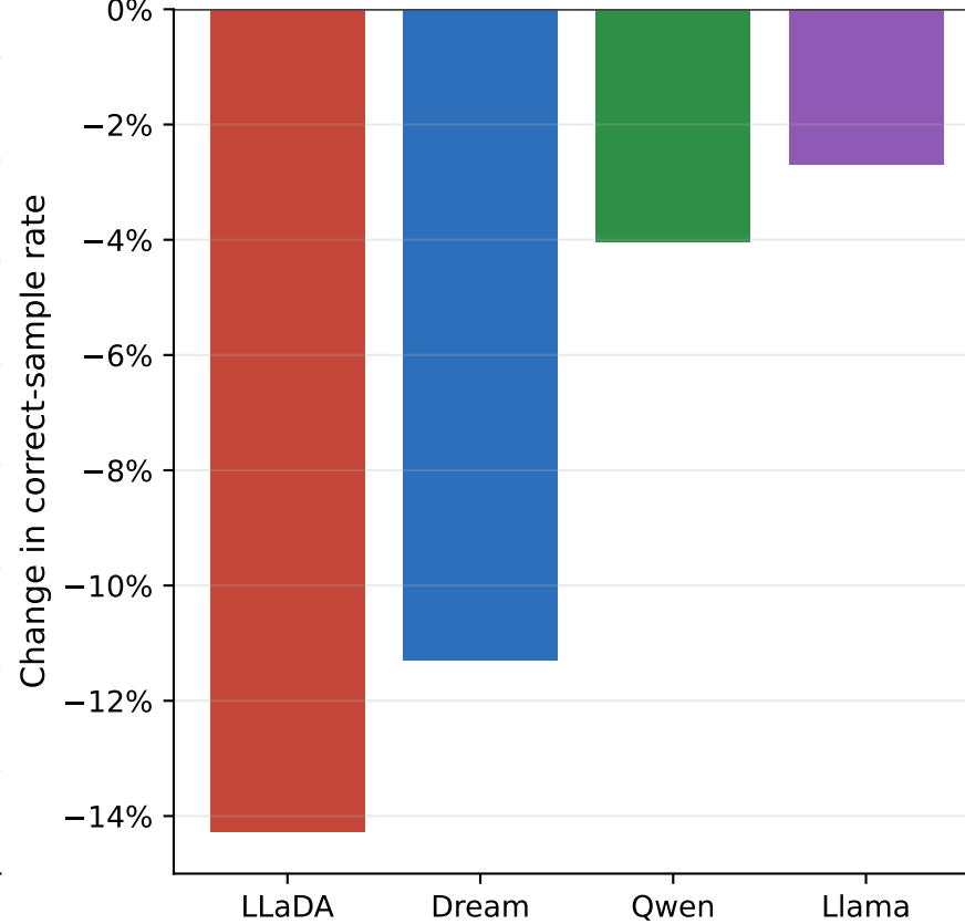
Countdown alternate-parser delta
