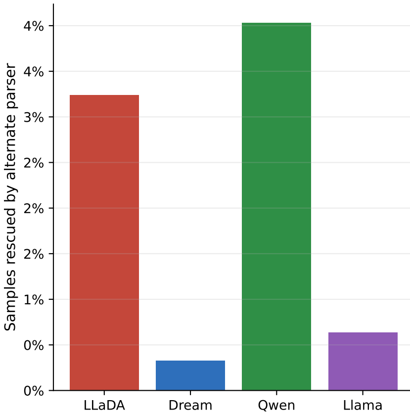
GSM8K box-only misses
