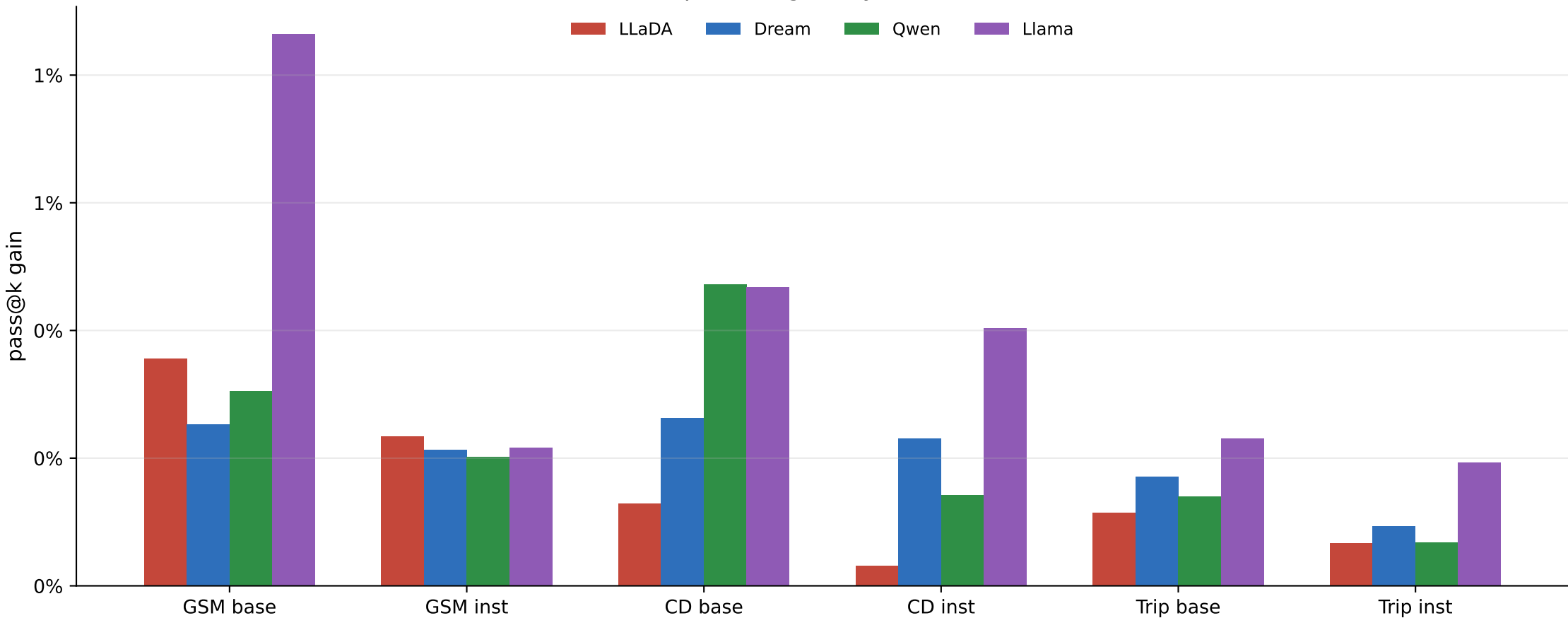
pass@k gain by model
