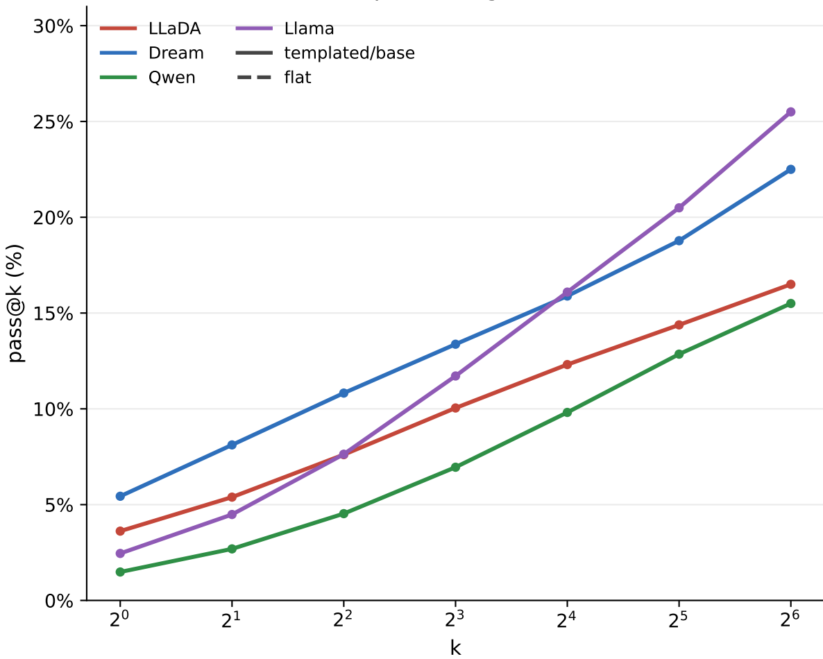
Trip Planning base
