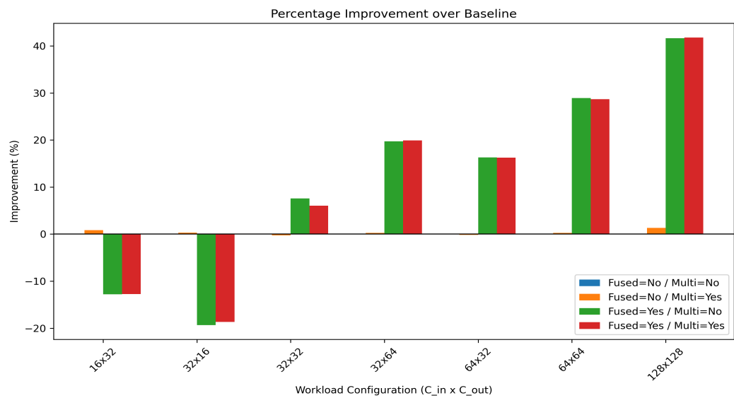
Figure 1: Percentage Latency Improvement/Regression relative to non-fused baseline across different workload shapes
