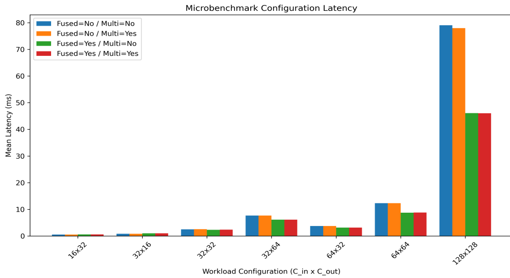
Figure 3: Absolute Latency (ms) comparison for Baseline vs Fused Winograd kernels
