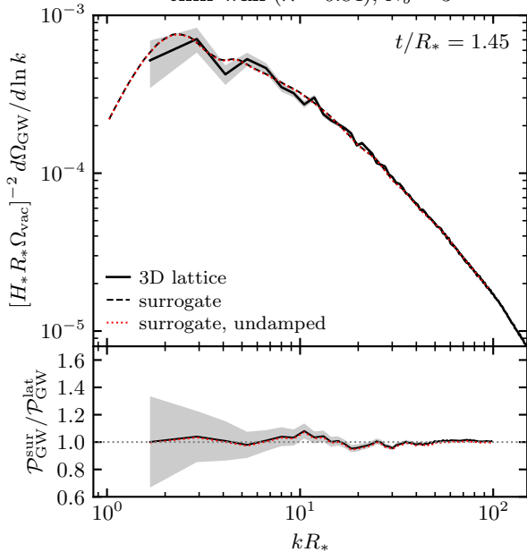
thin wall ( \bar{\lambda} = 0.84 ), N_b = 3
