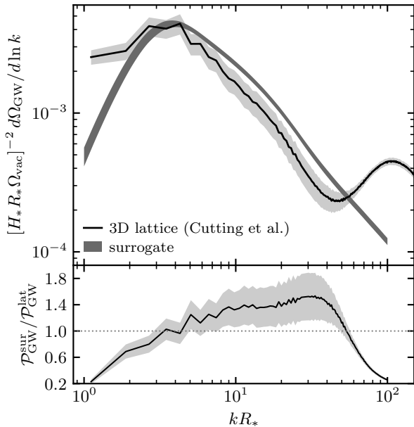
thin wall ( \bar{\lambda} = 0.845 ), \gamma_* = 4 , N_b = 512
