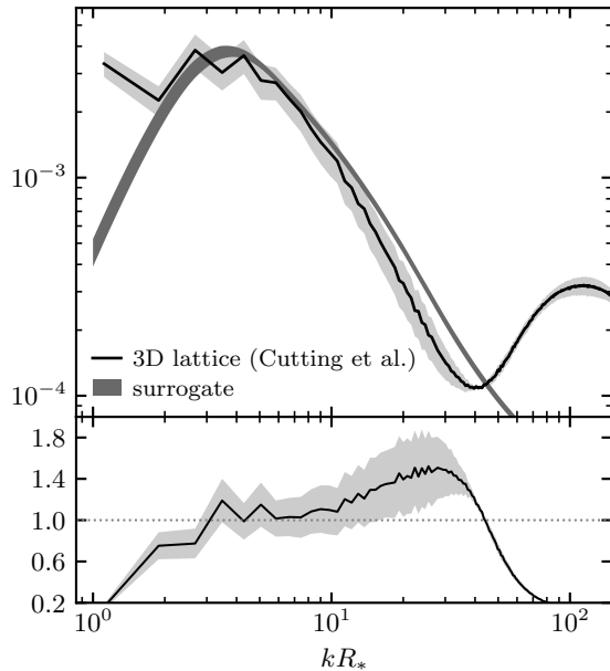
thick wall ( \bar{\lambda} = 0.069 ), \gamma_* = 4 , N_b = 512
