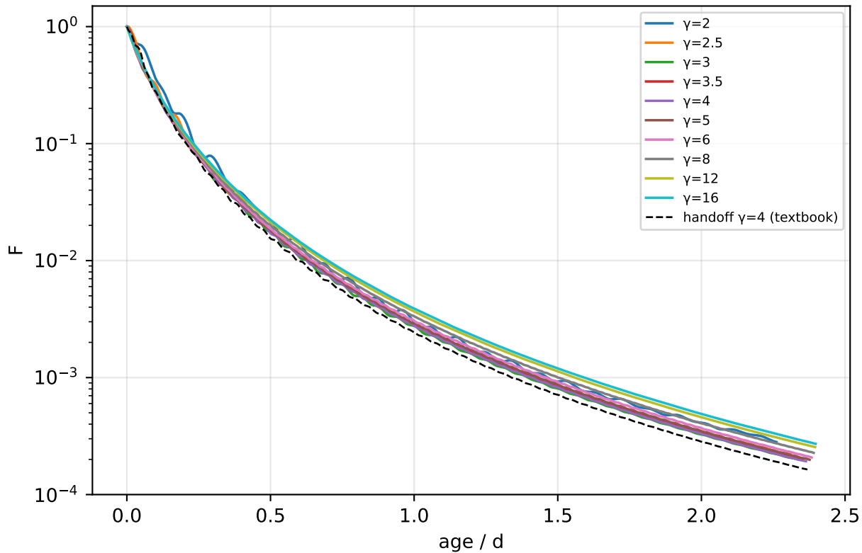
\bar{\lambda} = 0.84 , fixed_annulus, measured-wall calibration
