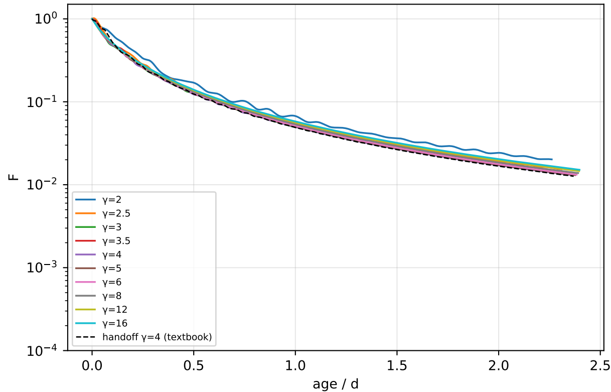
\bar{\lambda} = 0.84 , fixed_rapidity, measured-wall calibration
