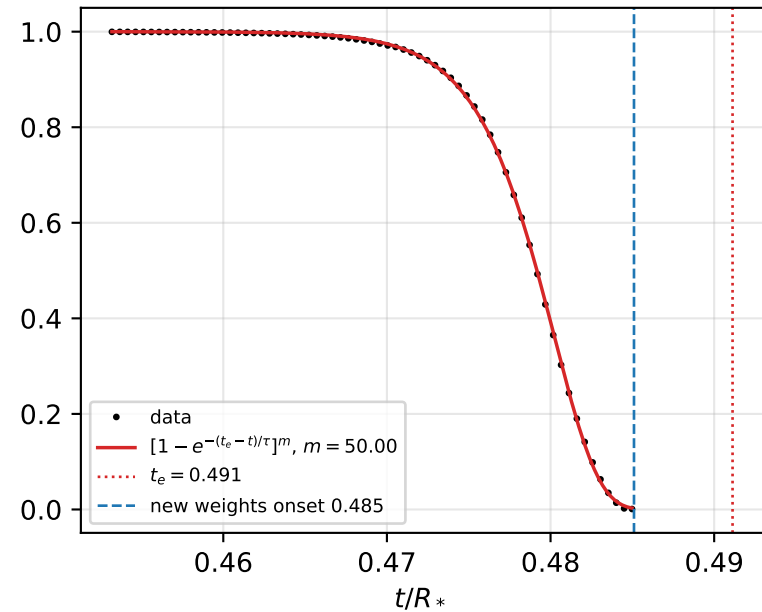
lb0.84_g4
