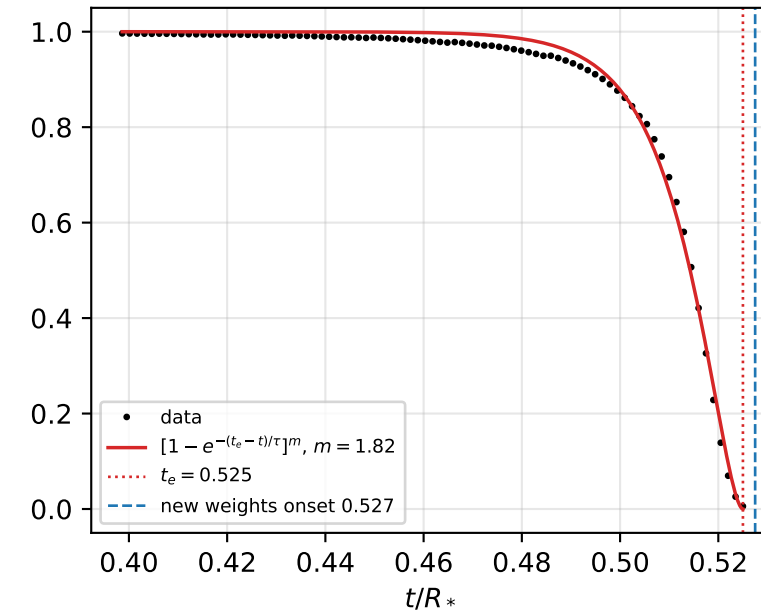
lb0.069_g4
