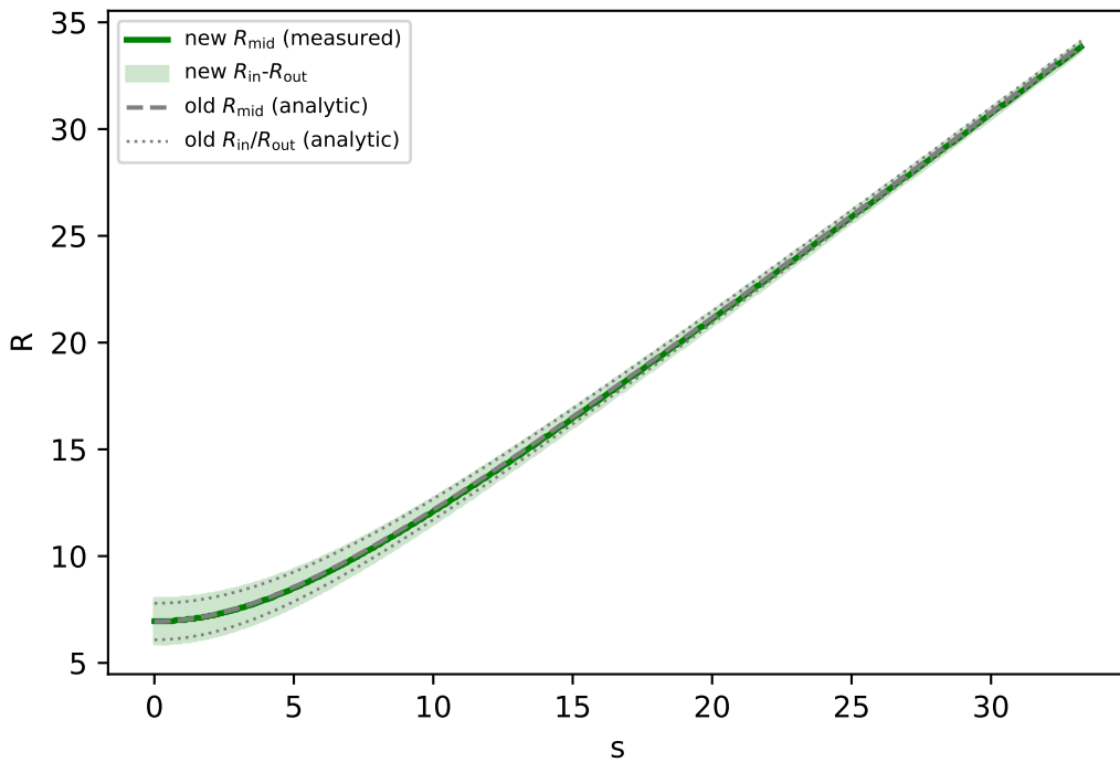
\bar{\lambda} = 0.069, \gamma = 2
