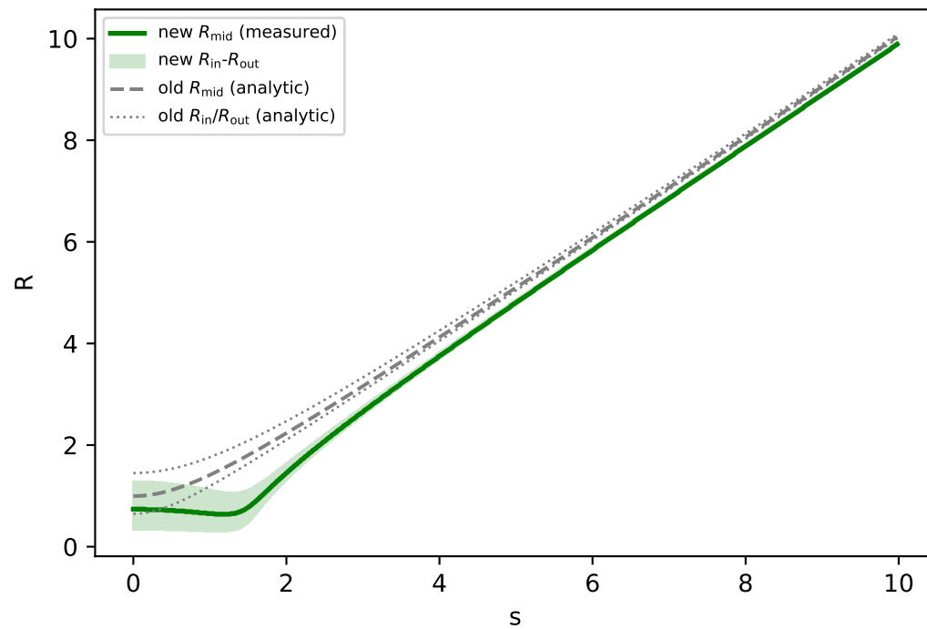
\bar{\lambda} = 0.069, \gamma = 4
