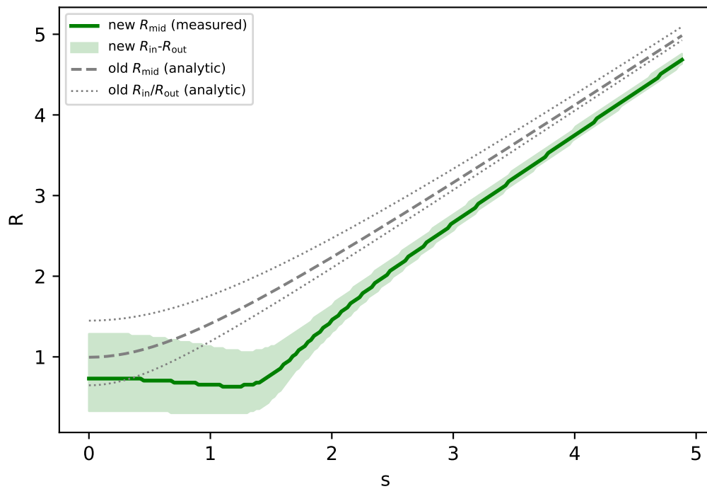
\bar{\lambda} = 0.069, \gamma = 2
