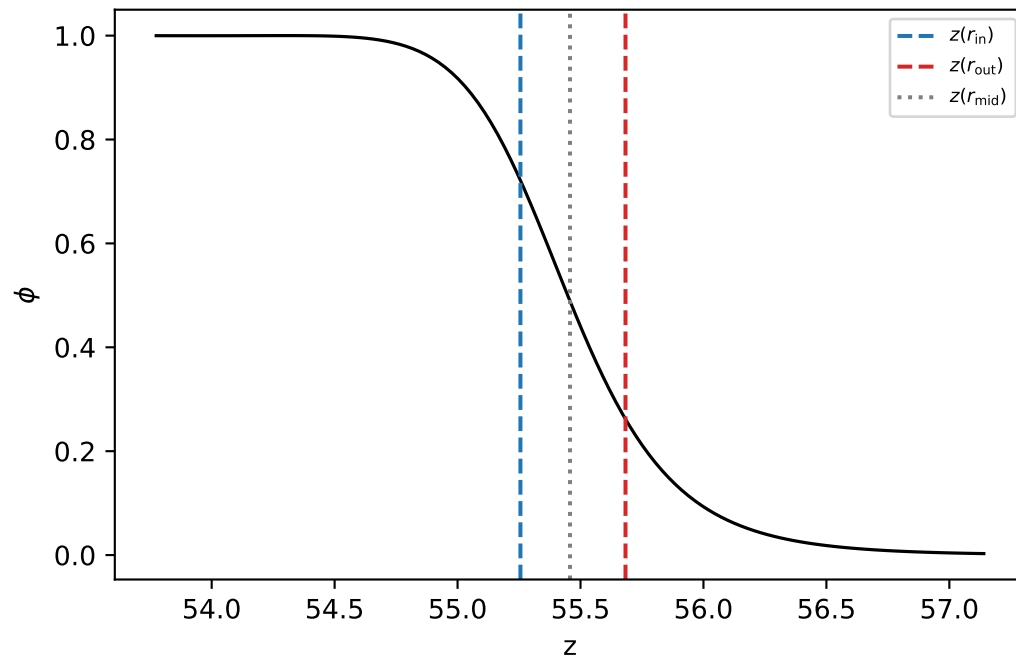
\bar{\lambda} = 0.84, \gamma = 4 s = 26.842 (requested t_{\text{coll}} = 26.847 ), local width = 0.4273
