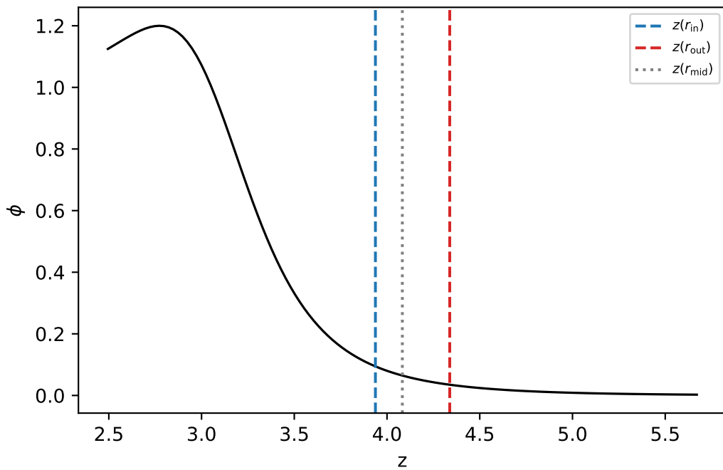
\bar{\lambda} = 0.069, \gamma = 2 s = 1.778 (requested t_{\text{coll}} = 1.782 ), local width = 0.4007
