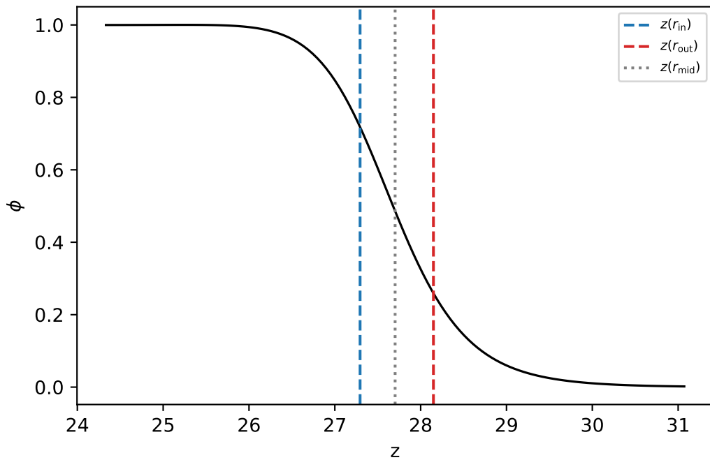
\bar{\lambda} = 0.84, \gamma = 2 s = 11.965 (requested t_{\text{coll}} = 11.989 ), local width = 0.8547
