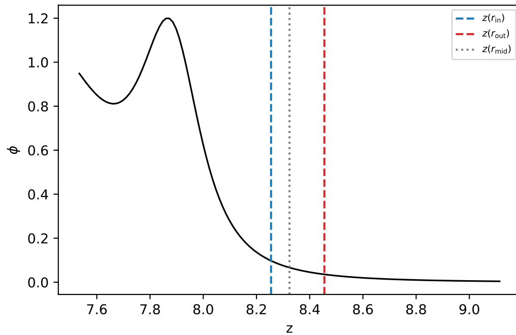
\bar{\lambda} = 0.069, \gamma = 4 s = 4.045 (requested t_{\text{coll}} = 4.041 ), local width = 0.2004
