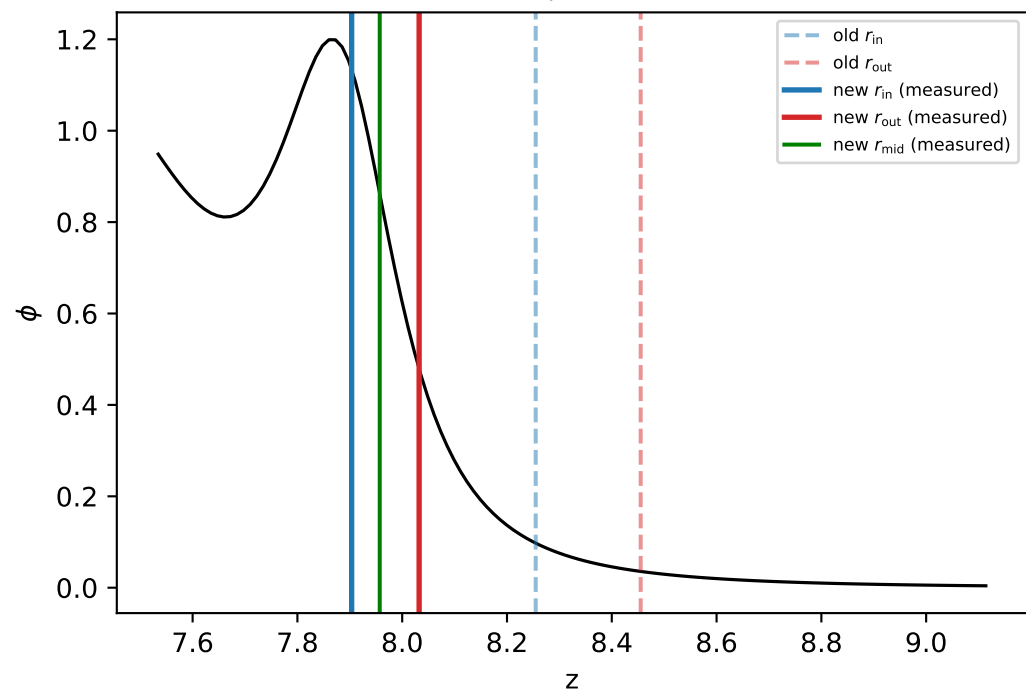
\bar{\lambda} = 0.069, \gamma = 4, s = 4.045
