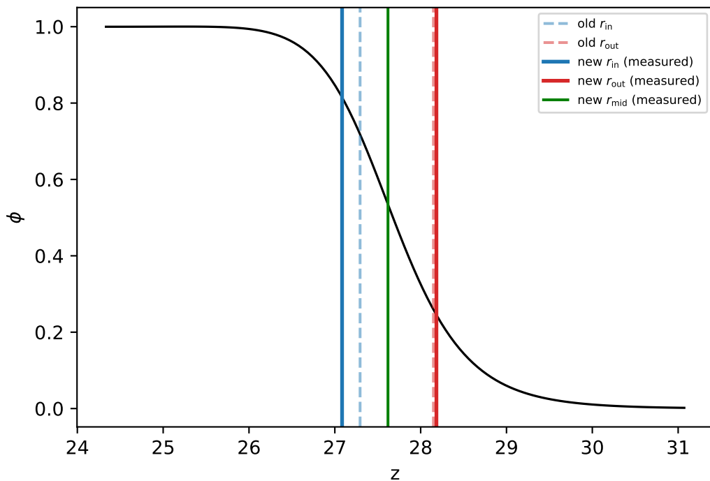
\bar{\lambda} = 0.84, \gamma = 2, s = 11.965
