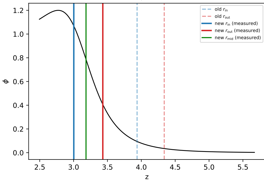
\bar{\lambda} = 0.069, \gamma = 2, s = 1.778
