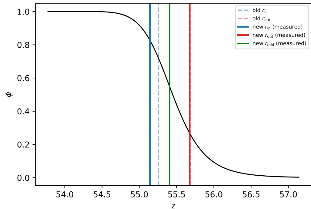
\bar{\lambda} = 0.84, \gamma = 4, s = 26.842
