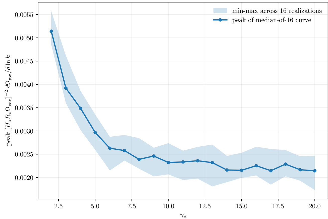
Peak spectral amplitude vs \gamma_* , \bar{\lambda} = 0.84
