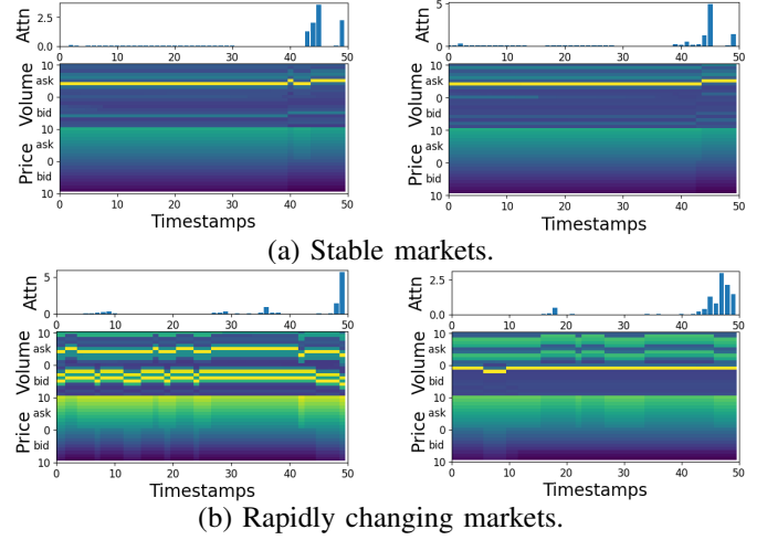
Fig. 3. Attention visualization.
