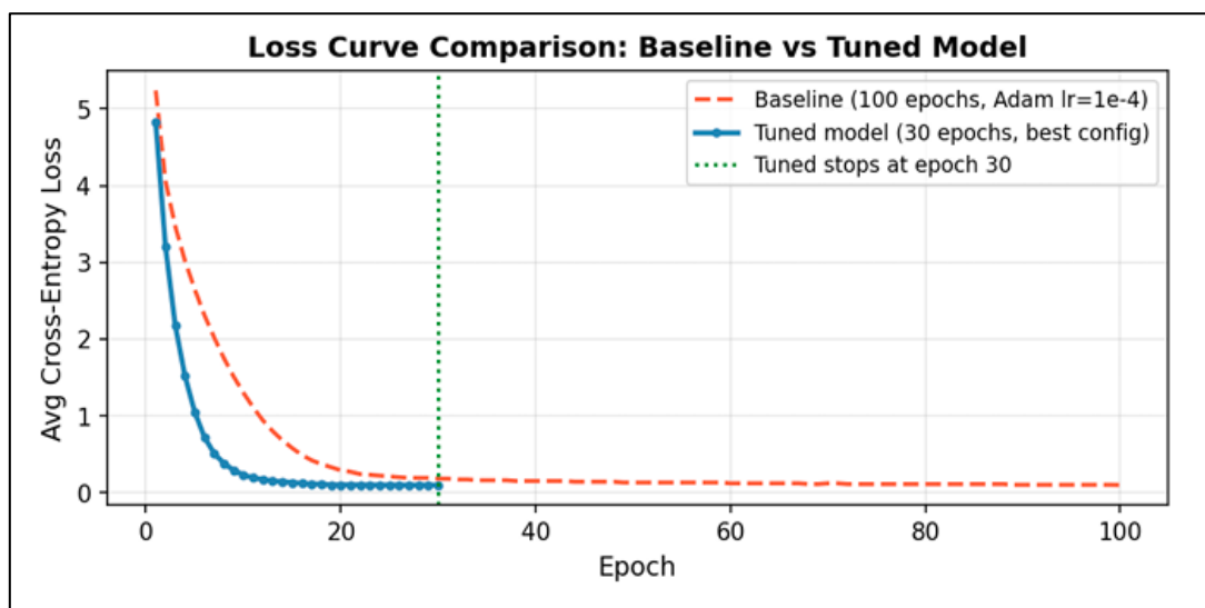
Fig(A). Loss Curve Comparison
