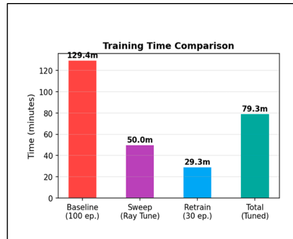
Fig(C). Training Time Breakdown
