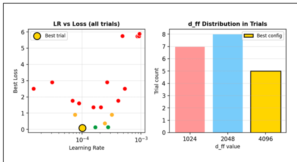
Fig(D). Hyperparameter Search Analysis
