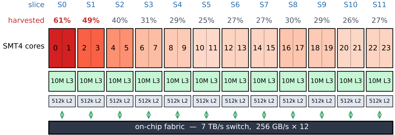
Fig. 1. POWER9 slice organisation (after [4]) annotated with the measured per-slice harvest rate across 1,960 Marconi100 sockets. Each slice holds two SMT4 cores sharing 512kB L2 and 10MB L3 on a common fabric port. Harvesting always removes whole slices. The horizontal ordering is the IPMI sensor index, which Sec. IV-F shows is the physical die ordering, recovered independently from thermal coupling.
