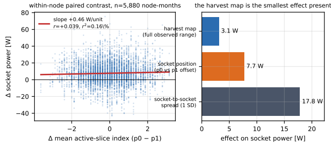
Fig. 11. Operational impact of the harvest map. Left: within-node paired contrast. Right: the harvest map’s full observed range moves socket power less than half as much as mere socket position, and a sixth as much as the socket-to-socket spread.
