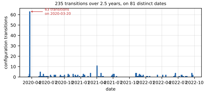
Fig. 10. Configuration transitions over the full record. 2020-03-20 alone accounts for 63.
