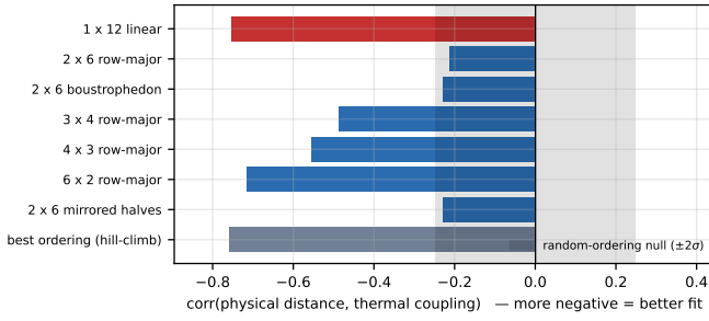
Fig. 5. Candidate floorplans scored against measured thermal coupling (more negative = better fit). The linear index ordering (red) wins decisively and is matched only by an unconstrained search that converges to the same arrangement reversed.
