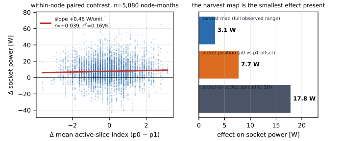
Fig. 12. Operational impact of the harvest map. Left: within-node paired contrast. Right: the harvest map's full observed range moves socket power less than half as much as mere socket position, and a sixth as much as the socket-to-socket spread.
