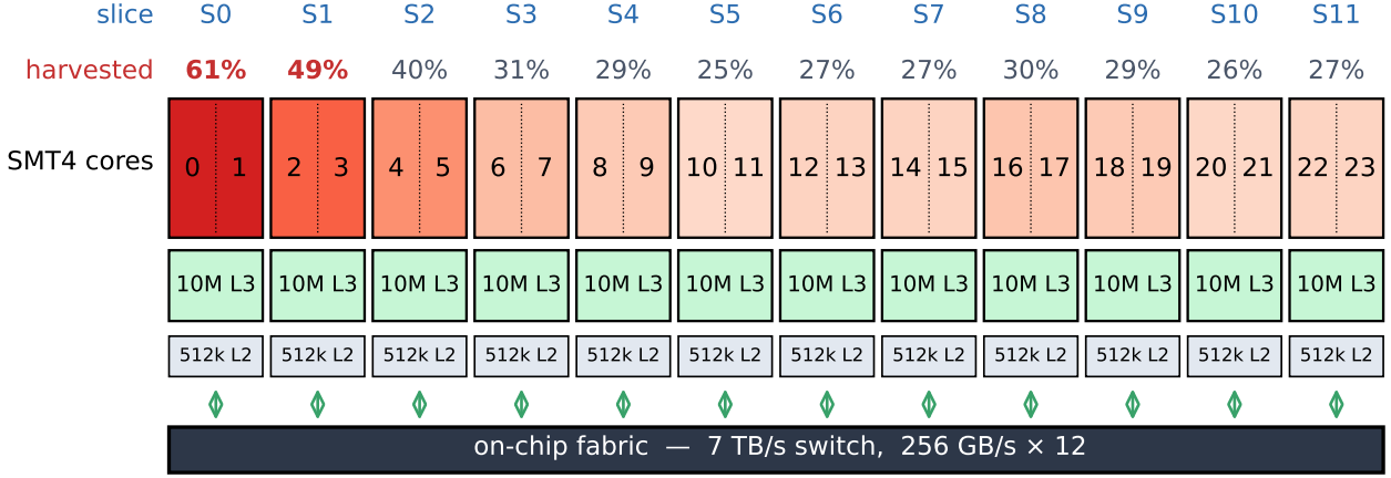
Fig. 2. POWER9 slice organisation (after [5]) annotated with the measured per-slice harvest rate across 1,960 Marconi100 sockets. Each slice holds two SMT4 cores sharing 512kB L2 and 10MB L3 on a common fabric port. Harvesting always removes whole slices. The horizontal ordering is the IPMI sensor index, which Sec. IV-F shows is the physical die ordering, recovered independently from thermal coupling.
