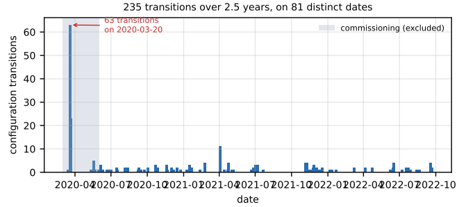
Fig. 11. Configuration transitions over the full record. 2020-03-20 alone accounts for 63, all inside the commissioning window (shaded) that Sec. IV-Hof excludes; the steady-state period shows no comparable cluster.
