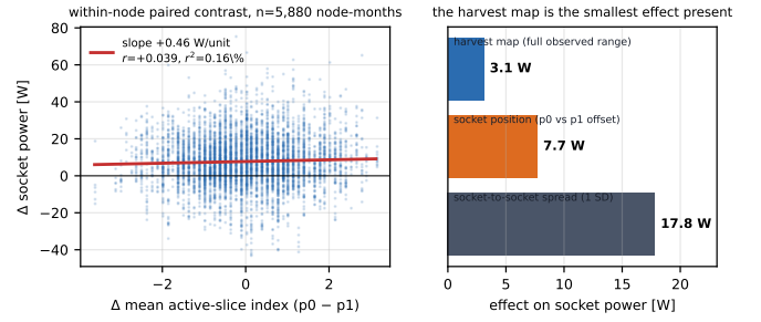
Fig. 12. Operational impact of the harvest map. Left: within-node paired contrast. Right: the harvest map's full observed range moves socket power less than half as much as mere socket position, and a sixth as much as the socket-to-socket spread.
