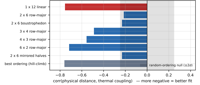
Fig. 6. Candidate floorplans scored against measured thermal coupling (more negative = better fit). The linear index ordering (red) wins decisively and is matched only by an unconstrained search that converges to the same arrangement reversed.
