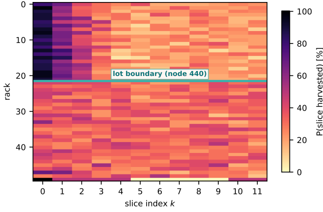
Fig. 7. Harvest probability by rack (rows: the 49 physical cabinets, 20 nodes each, in installation-id order) and slice (columns: position on the die). The procurement boundary is visible as an abrupt change across the whole die at once—the signature of a different population of parts, not of a room effect.
