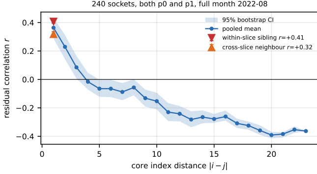
Fig. 4. Residual thermal correlation versus core index distance. The within-versus cross-slice contrast at distance 1 controls exactly for index gap.
