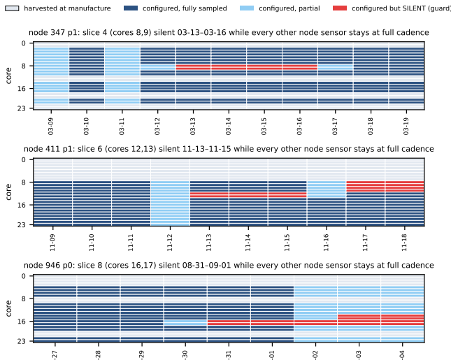
Fig. 9. The three core-guard episodes. Grey = harvested at manufacture, blue = configured and reporting, red = configured but silent. In every case exactly one slice goes silent while all ten control sensors on the same node stay at full cadence.
