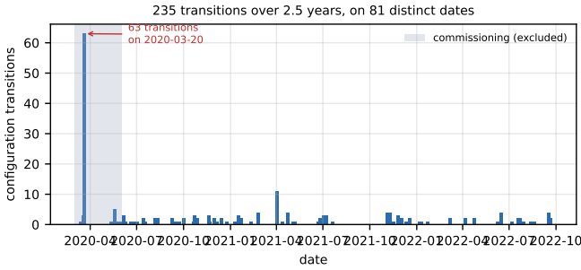
Fig. 10. Configuration transitions over the full record. 2020-03-20 alone accounts for 63, all inside the commissioning window (shaded) that Sec. IV-H0f excludes; the steady-state period shows no comparable cluster.
